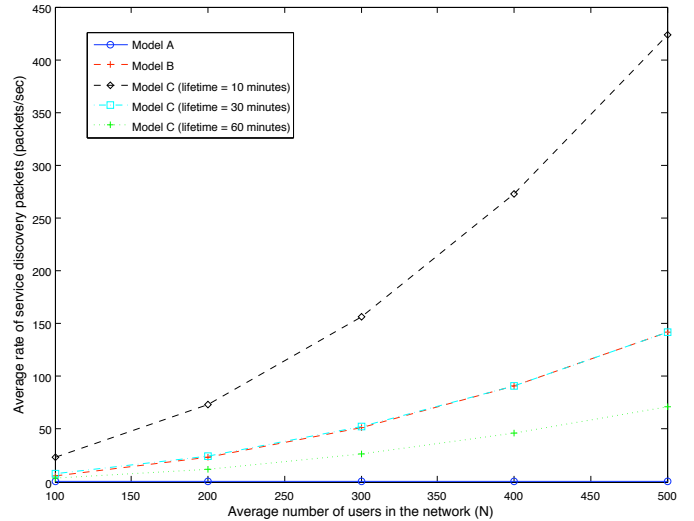
Fig. 6. The average service discovery packet rate of model A, B and C when period ( P ) is 30 minutes. The average rates are obtained from the Table III.
